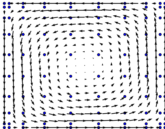
Fig. 9. Plot for the solution of (\star \mathbf{d} \star \mathbf{d} + \mathbf{d} \star \mathbf{d} \star) f = 0 with the boundary conditions of \star f|_B = 0 (vector field is tangent to the boundary) and \mathbf{d} \star f|_B = 1 (the curl at the boundary is equal to 1). The domain is [-1, 1]^2 , discretized by a 10 \times 10 Chebyshev grid.
