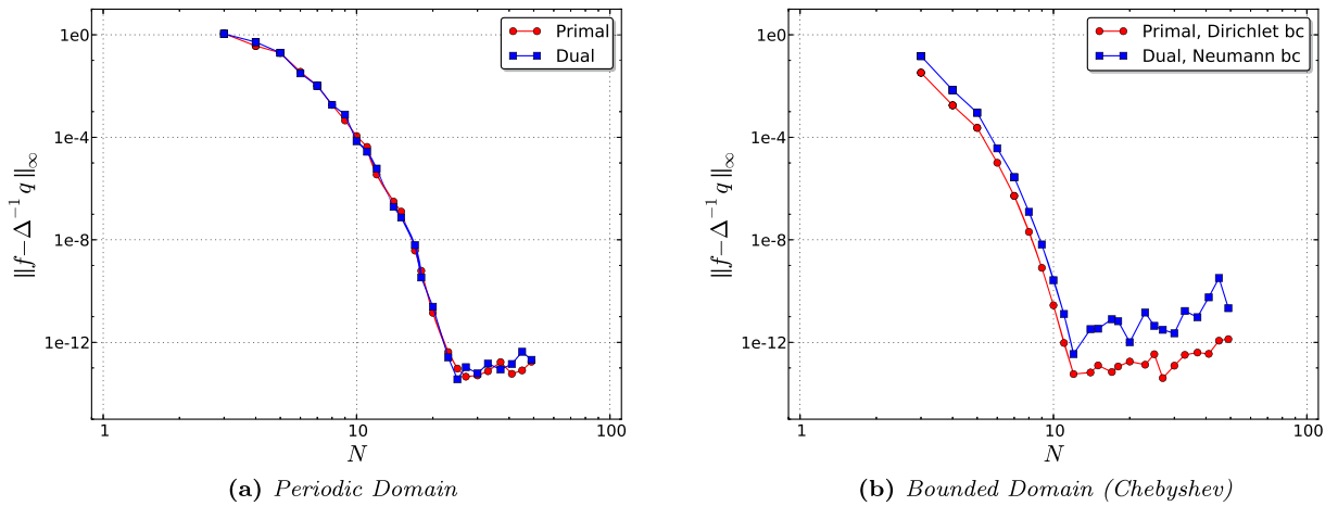
Fig. 7. Convergence graphs for a 1D Poisson equation: (a) we solve \Delta f = e^{\sin x}(\cos^2 x - \sin x) on a periodic domain for either a primal, or dual 0-form f ; (b) we solve \Delta f = e^x on a Chebyshev grid, for either a primal 0-form with Dirichlet boundary conditions f(-1) = e^{-1} and f(1) = e , or for a dual 0-form with Neumann boundary conditions f'(-1) = e^{-1} and f'(1) = e . All of our results exhibit spectral convergence (measured through the L^\infty error \|f - \Delta^{-1}q\|_\infty ), with the conventional plateau when we reach the limit of accuracy of the representation of floating point numbers.
